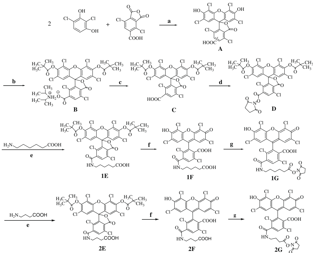
Scheme 1. Synthesis of two novel chlorinated fluorescein succinimidyl esters 1G and 2G . Reagents and conditions: (a) methyl sulfonic acid, N_2 , 48 h, 100 °C; (b) 1. pivalic anhydride, reflux; 2. diisopropylamine, anhyd alcohol; B yield: 38%; (c) 1 M HCl; C yield 93%; (d) NHS-TFA, pyridine, CH_2Cl_2 rt.; D yield 83%; (e) 6-aminohexanoic acid/4-aminobutanoic acid, CH_2Cl_2 rt. 1E yield 63%, 2E yield 67%; (f) (1) NH_3/H_2O ; (2) 1 M HCl; 1F yield 89%, 2F yield 93%; (g) NHS-TFA, pyridine, CH_2Cl_2 rt.; 1G yield 78%, 2G yield 82%.
