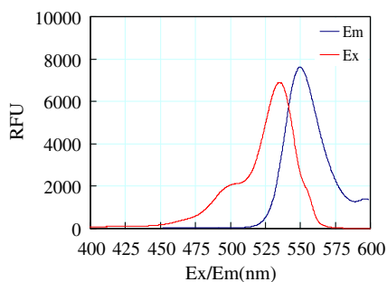
Figure 1. Excitation and emission spectrum of compound 1G in 0.1 M NaOH.
