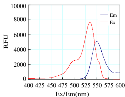
Figure 2. Excitation and emission spectrum of compound 2G in 0.1 M NaOH.
